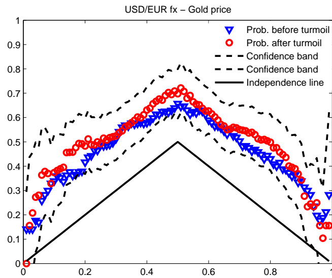
Figure 7: Estimated tail co-dependence
