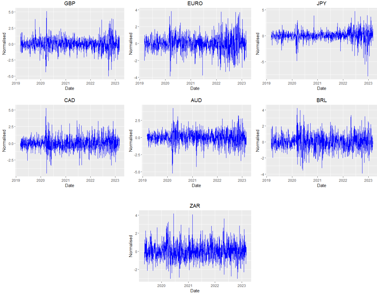
Figure 5: Normalised Exchange Rates. y_t was normalised by subtracting its mean and dividing by the standard deviation. The x-axis plots the dates that correspond to the end of each year for the daily observations. The y-axis plots the normalised y_t
