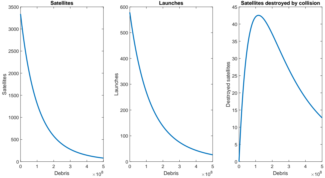
Figure 1: Satellites, launches and satellites destroyed in steady state by collision as a function of debris
