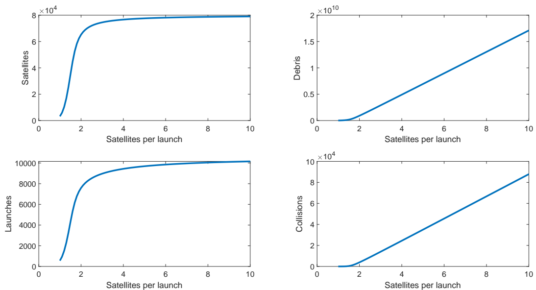
Figure 5: Steady state as a function of the number of satellites per launch.
