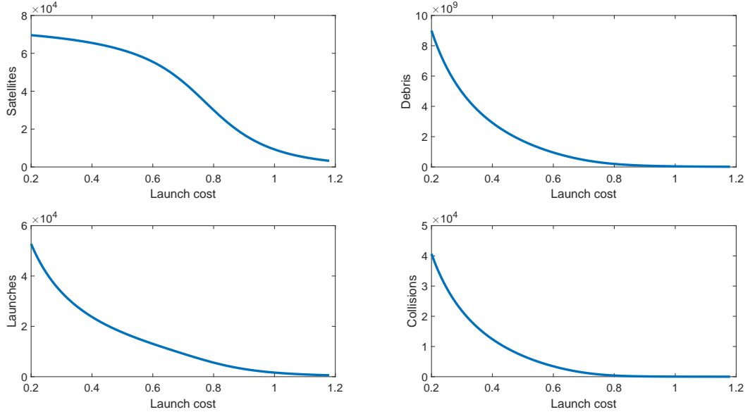
Figure 4: Steady state values as a function of the launch cost.
